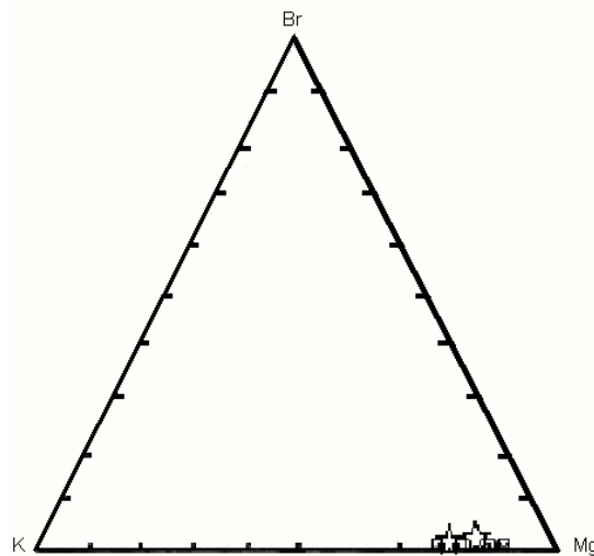
Figure 6. Composition of fluid inclusions compared to the one of mother brines of halite crystals
