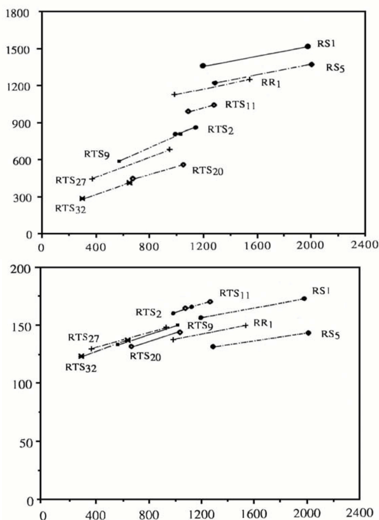
Figure 5. Diagrams showing the reduction of contents in Br, K and Mg in halite crystals after their grinding in the ethanol
