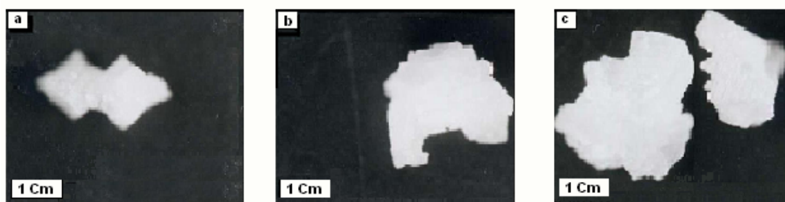
Figure 3. Different shapes of halite crystal observed in crystallizers of Sfax saline. a: Hoppers shape b: Inverse pyramids shape c: Chevrons shape
