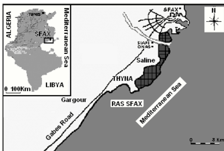
Figure 1. Location map of Sfax saline (S.E Tunisia)
