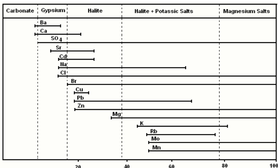
Figure 7. Sequence of crystallisation of some chemical elements during the evaporation Of seawater (according to AMDOUNI [1])
