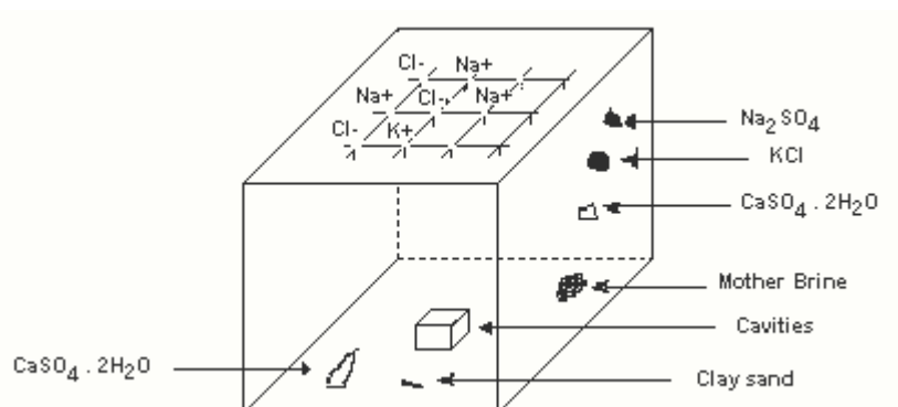
Figure 4. Different types of Impurities that can be met in crystals of halite (according to MASUZAWA [3])
